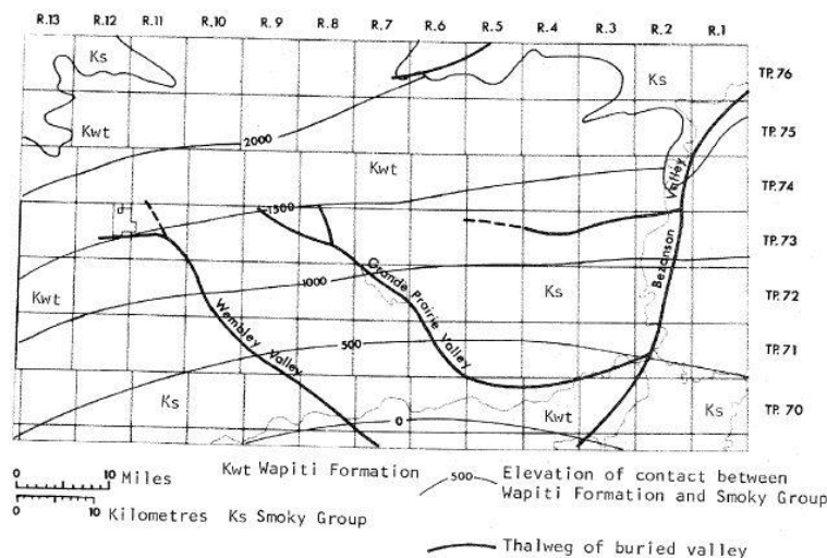
Figure 11. Buried Valleys near Grande Prairie [Hackbarth, 1978]
