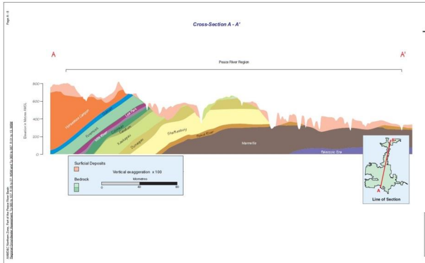
Figure 5. Upper Bedrock Cross Sections of Western Basins. [HCL, 2004]
