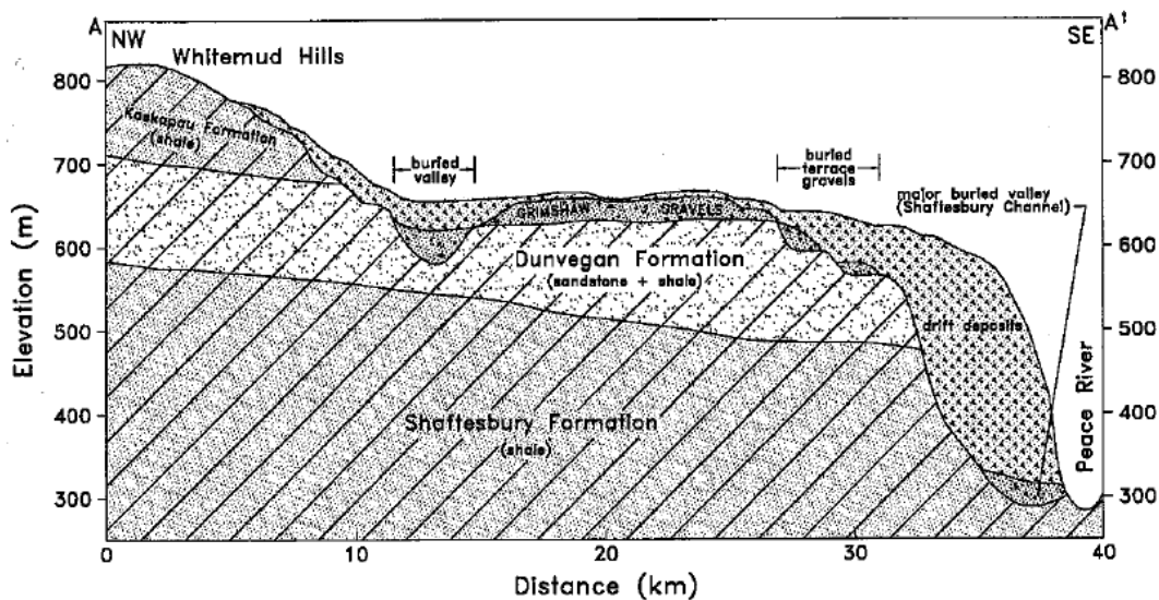
Figure 12 Cross Section of Grimmshaw Gravel [PFRA, 1998]
