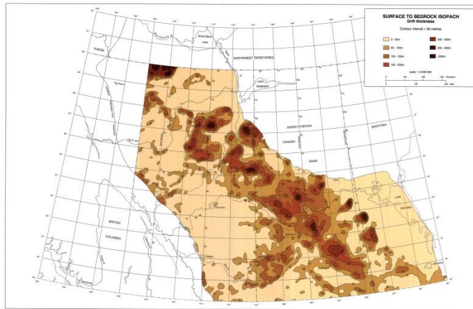
Figure 2. Surficial Sediment Thickness where [Alberta Geologic Survey, 1998]
