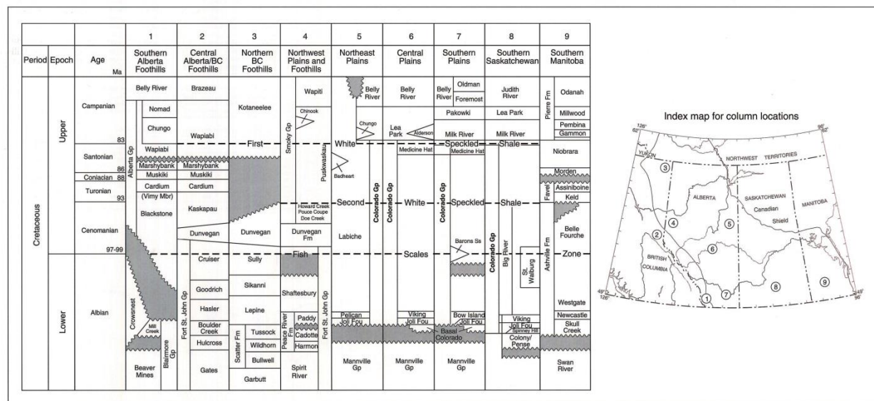
Figure 20.1 Stratigraphic terminology of the Colorado/Alberta Group.
