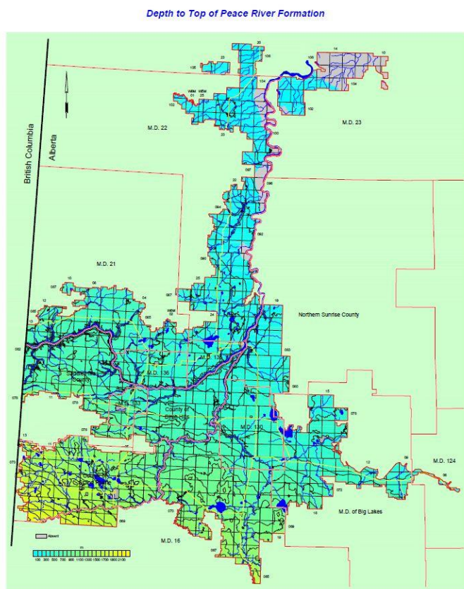
Figure 8. Depth to Top of Peace River Formation [HCL, 2004]
