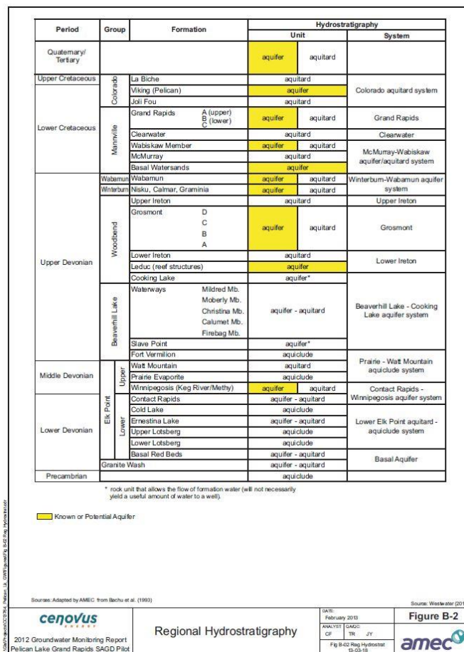
Figure 9. Stratigraphic Column from the Pelican Lake Area of Alberta. [AMEC, 2012]
