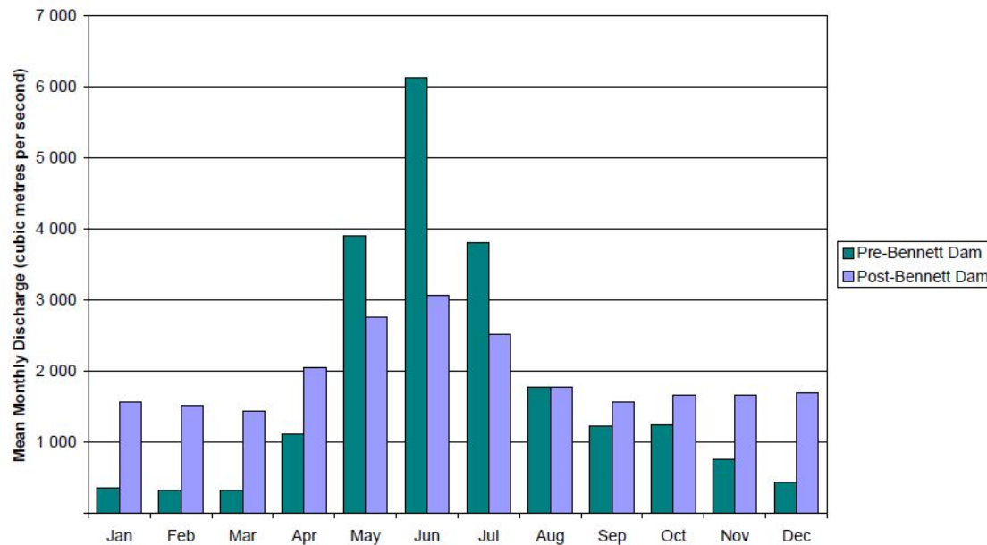
Figure 10. Changes of Annual Flow Due to Bennett Dam. [M.Seneka, AENV, 2004]
