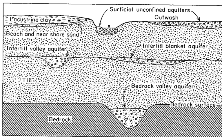
Figure 1. Schematic diagram of aquifer occurrence in glaciated regions. [Freeze&Cherry, 1979]
