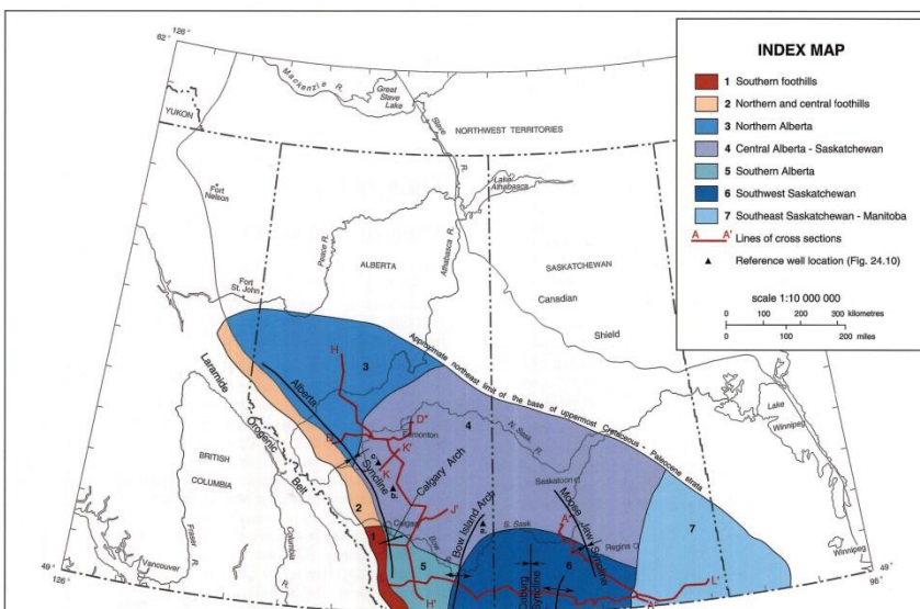
Figure 4. Major Structural Geology Features, Alberta Geologic Survey, 1998
