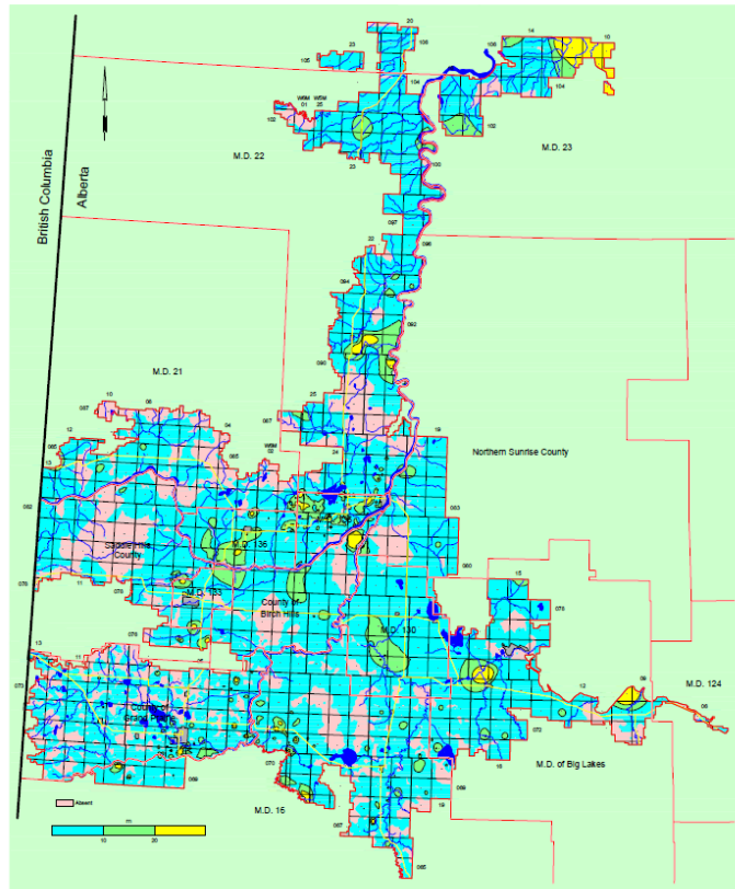
Figure 3. Thickness of Sand and Gravel in Drift (m), Western Basins [HCL, 2004]
